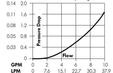
Pressure Drop - High Flow
