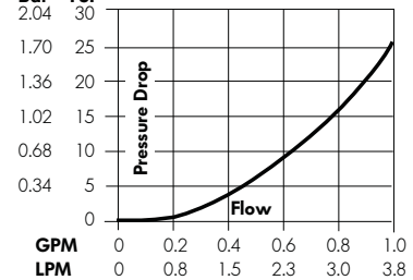
Pressure Drop - High Flow
